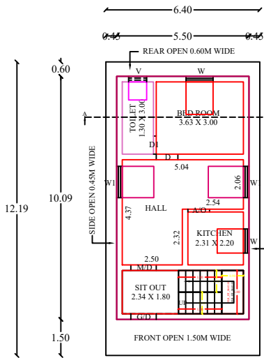
GROUND FLOOR PLAN (SOUTH FACING)
