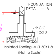
Isolated Footing - A (1.50X1.50) (Not To Scale)
