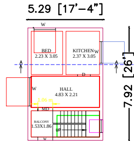
FIRST FLOOR PLAN (PROPOSED)
