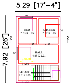
GROUND FLOOR PLAN (EXISTING)
