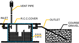
SEPTIC TANK & D-TRENCH DETAILS
