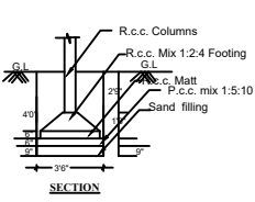
SECTION ON "AA"
