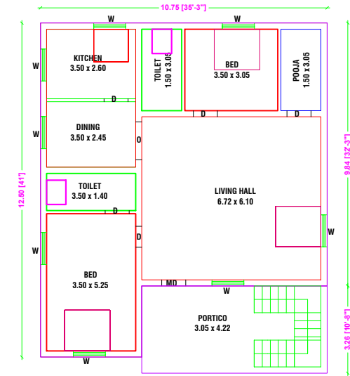
PRO.GROUND FLOOR PLAN NORTH FACING
