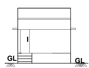
FRONT ELEVATION
