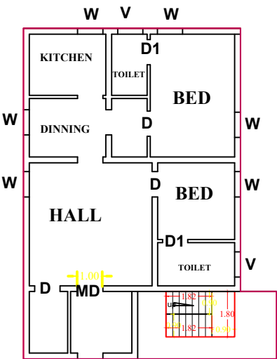
EXIST GROUND FLOOR PLAN
