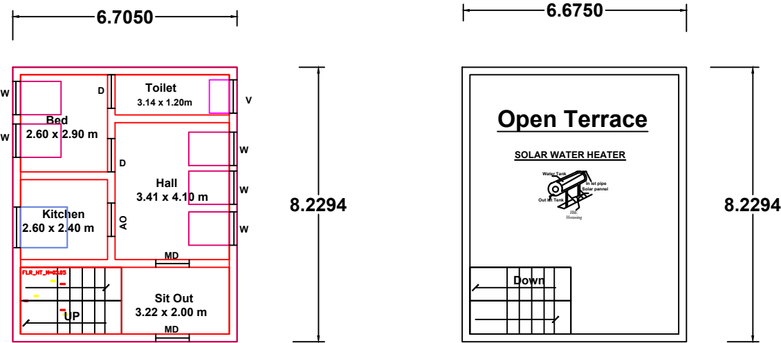
GROUND FLOOR PLAN ( NORTH FACING )
