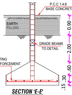
SECTION 'E-E'
