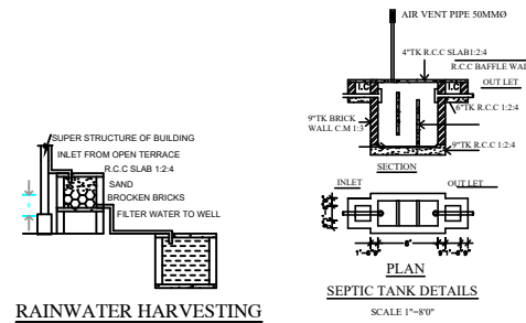
RAINWATER HARVESTING
