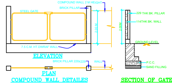
SECTION OF GATE
