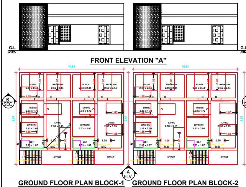
GROUND FLOOR PLAN BLOCK-1 GROUND FLOOR PLAN BLOCK-2
