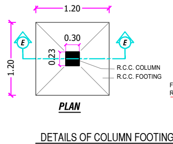
DETAILS OF COLUMN FOOTING
