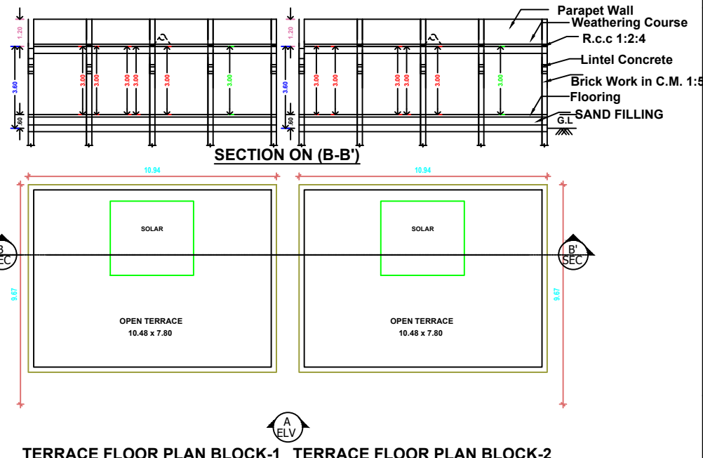
TERRACE FLOOR PLAN BLOCK-1 TERRACE FLOOR PLAN BLOCK-2
