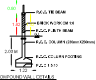
— 1.22 — COMPOUND WALL DETAILS
