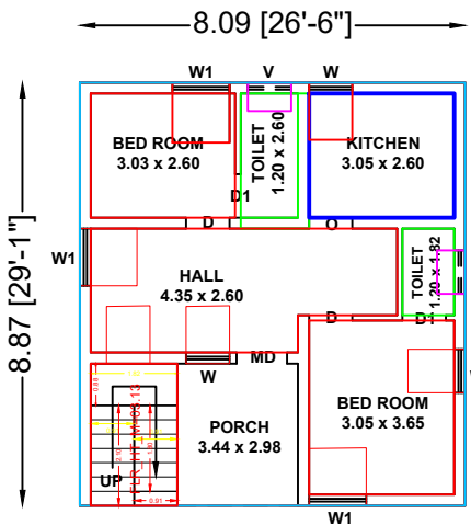
GROUND FLOOR PLAN (WEST FACING)
