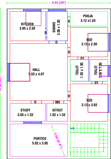
PRO. GROUND FLOOR PLAN NORTH FACING
