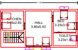
GROUND FLOOR PLAN ( NORTH FACING)
