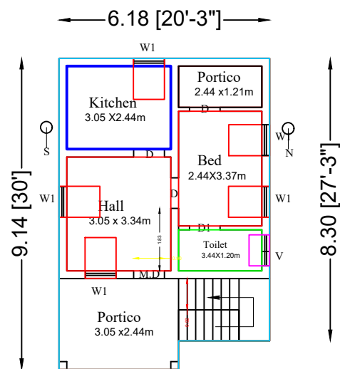
Ground Floor Plan (North Face)
