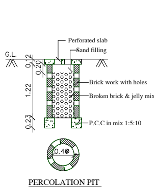
PERCOLATION PIT
