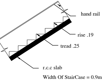
STAIRCASE DETAILS
