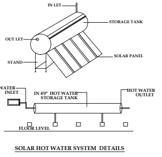
SOLAR HOT WATER SYSTEM DETAILS
