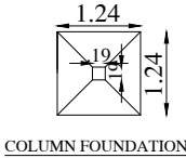
COLUMN FOUNDATION
