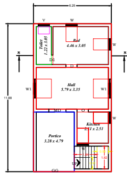
Exist Ground Floor Plan South facing
