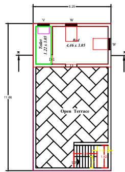
Proposed First Floor Plan
