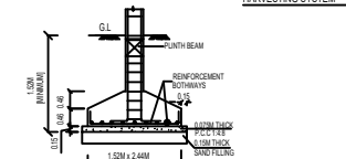
TYP. DET. COLUMN & FOUNDATION FOOTING
