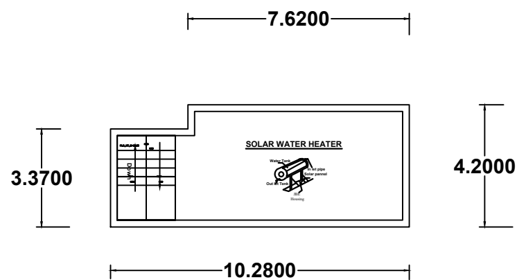
OPEN TERRACE
