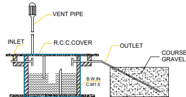
SEPTIC TANK & D-TRENCH DETAILS
