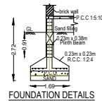
FOUNDATION DETAILS
