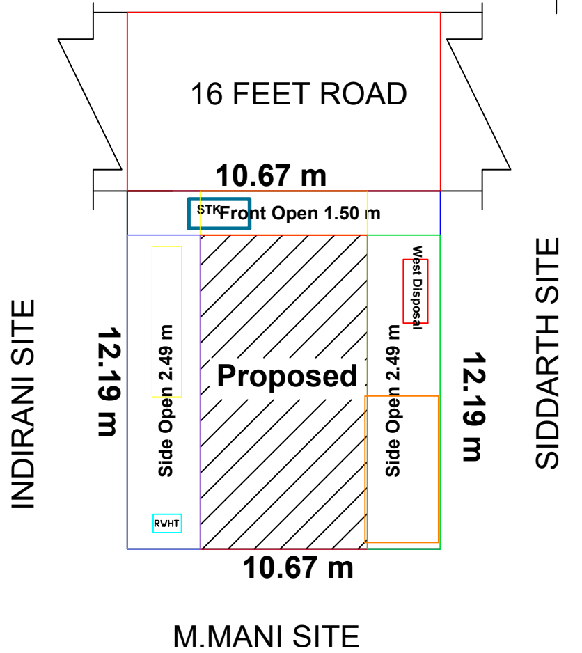
SITE PLAN
