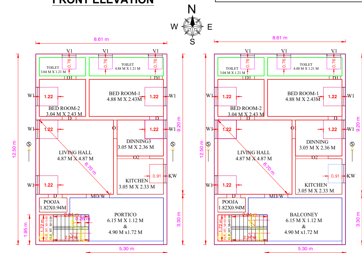
GROUND FLOOR PLAN [SOUTH FACING]
