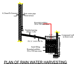
PLAN OF RAIN WATER HARVESTING
