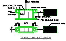
RainWater Harvesting Tank
