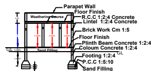
SECTION SECTION - AB
