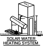
SOLAR WATER HEATING SYSTEM
