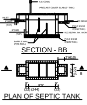
SECTION - BB
