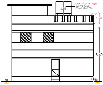
FRONT ELEVATION ( SOUTH FACING )
