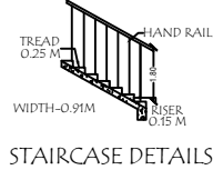
STAIRCASE DETAILS
