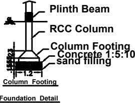
Column Footing
