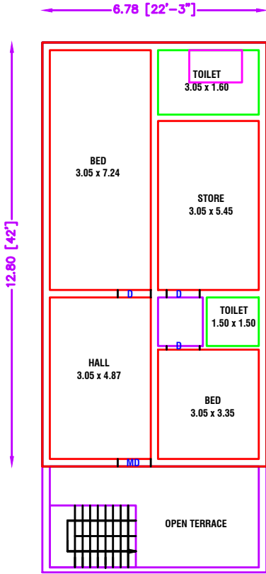
FIRST FLOOR PLAN [EAST FACING]
