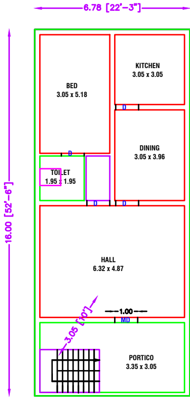
GROUND FLOOR PLAN [EAST FACING]
