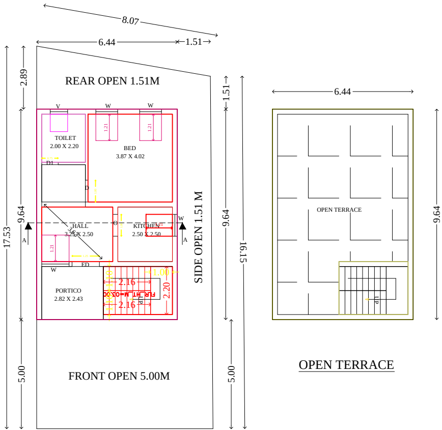
GROUND FLOOR (SOUTH FACING)
