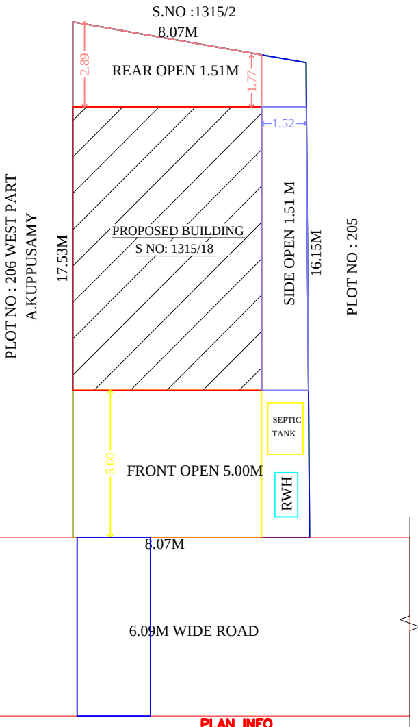
SITE PLAN
