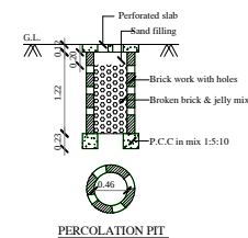
PERCOLATION PIT
