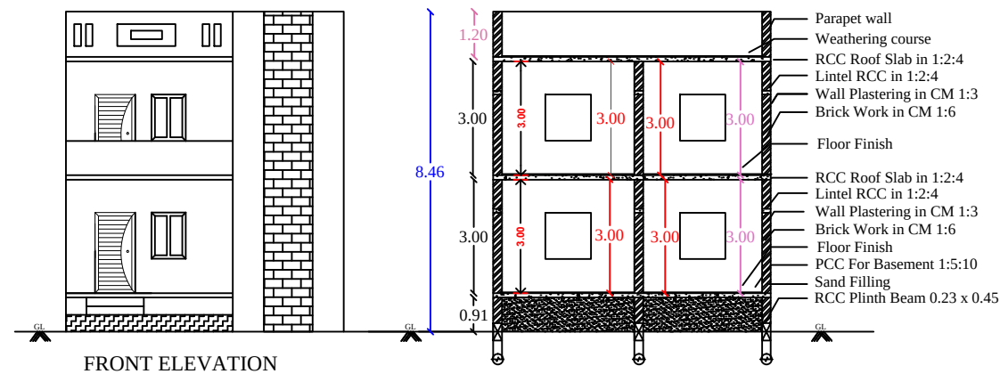
FRONT ELEVATION
