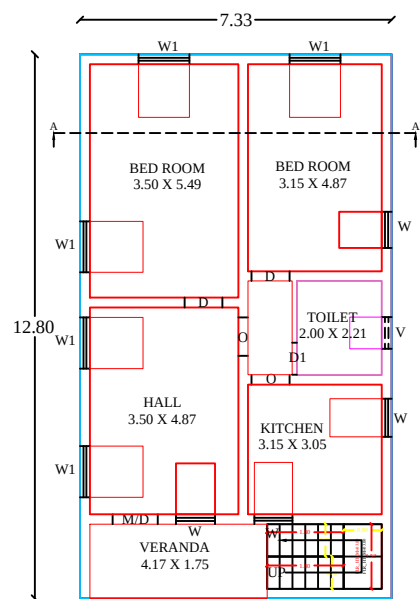
GROUND FLOOR PLAN (SOUTH FACING)
