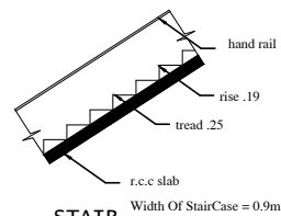
STAIR
