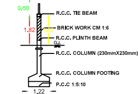
COMPOUND WALL DETAILS
