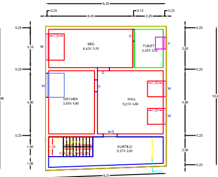
PROPOSED GROUND FLOOR PLAN (EAST FACING)
