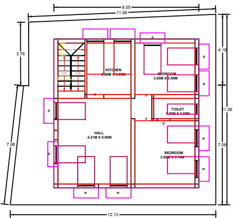
GROUND FLOOR PLAN ( WEST FACING)
