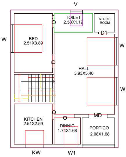
PRO. GROUND FLOOR
