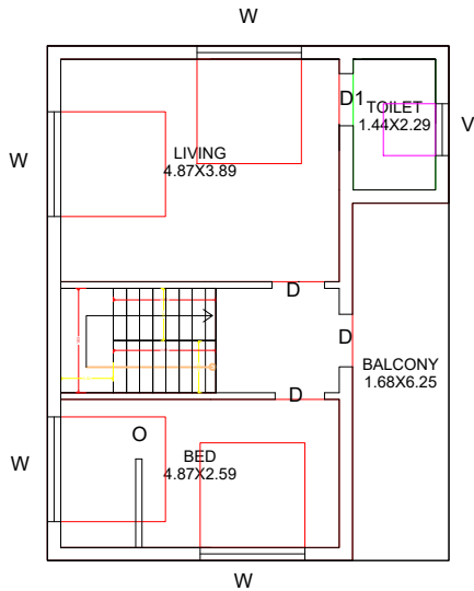
PRO FIRST FLOOR
