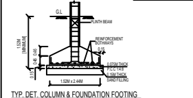
TYP. DET. COLUMN & FOUNDATION FOOTING
