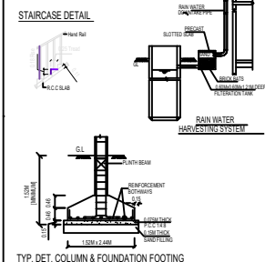
TYP. DET. COLUMN & FOUNDATION FOOTING
