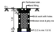
PERCOLATION PIT FOR 30sq.m. (Scale:- 1:50)
