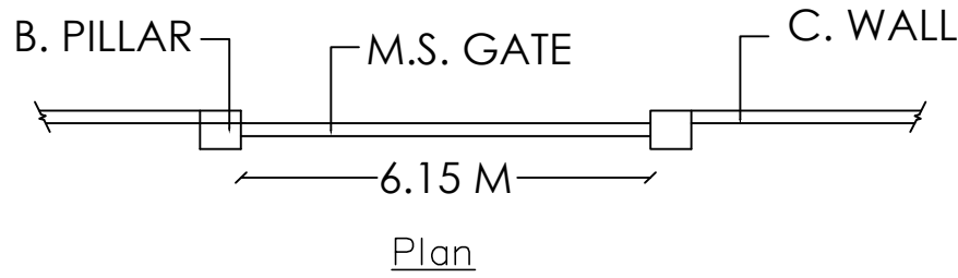
Compound Wall & Gate Details
