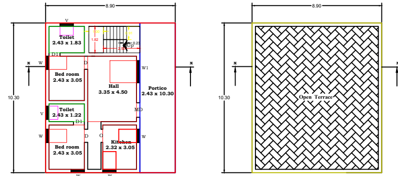
Proposed Ground Floor Plan (East Facing )
