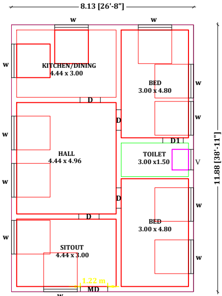
GROUND FLOOR PLAN NORTH FACING
