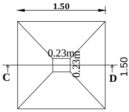
SECTION - 'CD'
