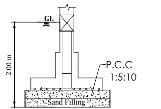
FOUNDATION DETAIL - A
