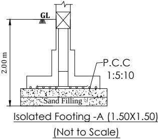
FOUNDATION DETAIL - A
