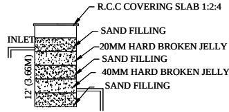
RAIN WATER HARVESTING
