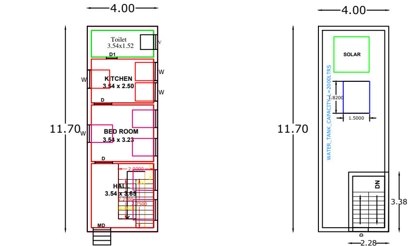
GROUND FLOOR PLAN ( NORTH FACING)
