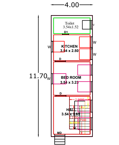
GROUND FLOOR PLAN ( NORTH FACING)
