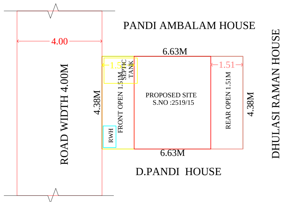
SITE PLAN
