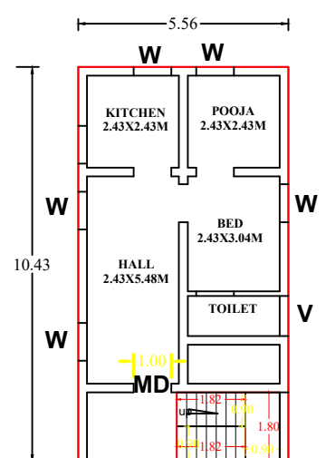
EXIS GROUND FLOOR PLAN
