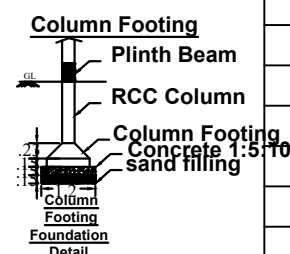
Column Footing Detail
