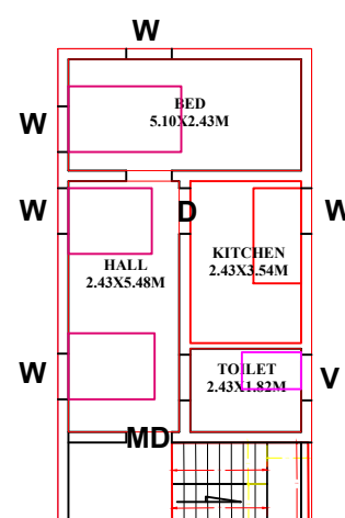
PRO FIRST FLOOR PLAN
