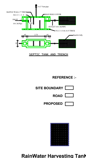
RainWater Harvesting Tank
