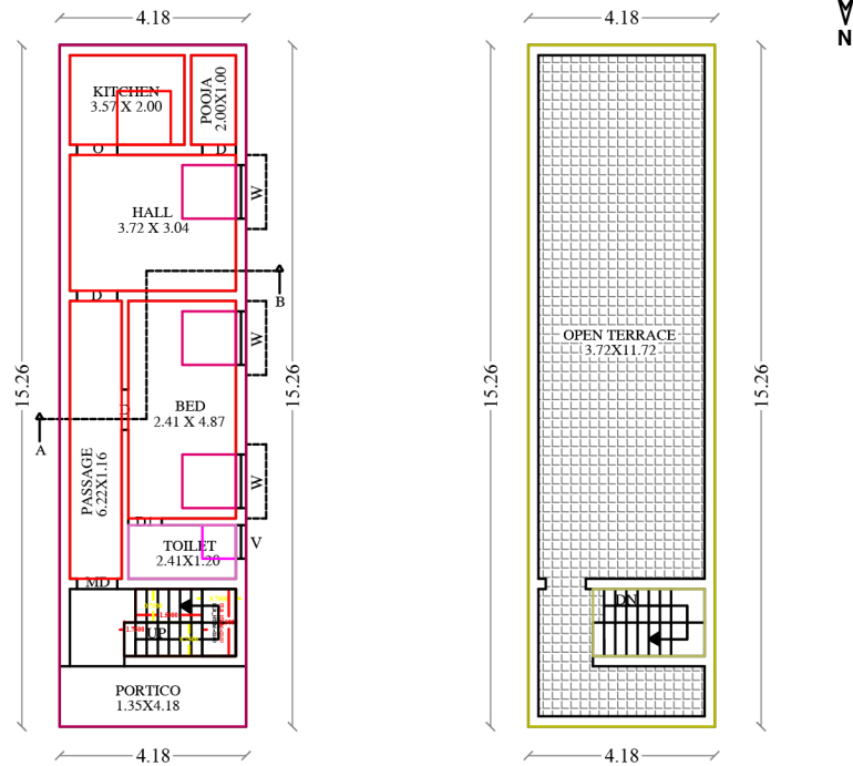
TERRACE FLOOR
