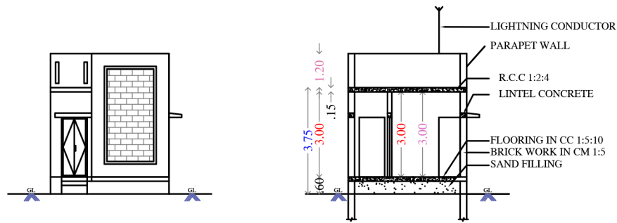
SECTION AB
