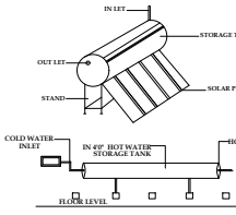
SOLAR HOT WATER SYSTEM DETAILS
