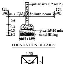
COLUMN FOUNDATION
