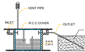
SEPTIC TANK & D-TRENCH DETAILS
