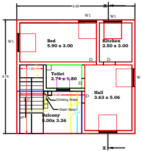
Proposed Basement Floor 2 Plan
