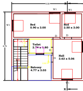
Proposed Basement Floor 1 Plan
