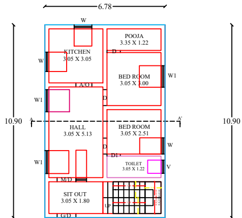
GROUND FLOOR PLAN (NORTH FACING)
