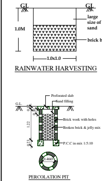
PERCOLATION PIT
