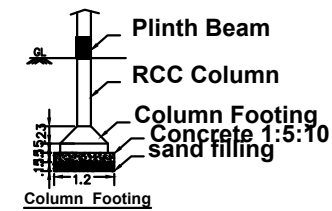
Foundation Detail
