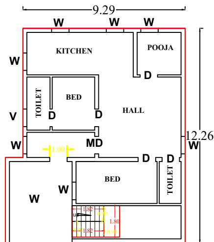
EXIS GROUND FLOOR PLAN
