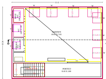
EXISTING GROUND FLOOR (WEST FACING)
