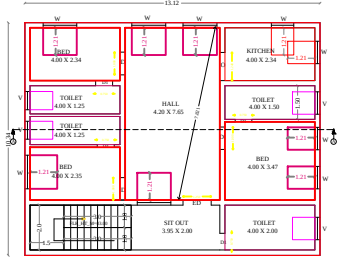
FIRST FLOOR (WEST FACING)
