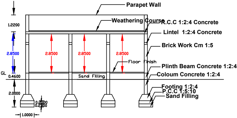
Section Section - AA
