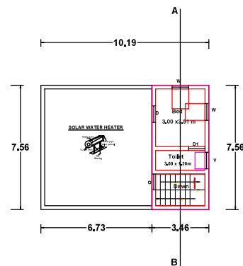
PROPOSED FIRST FLOOR & OPEN TERRACE
